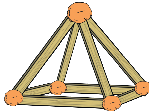
square-based pyramid
